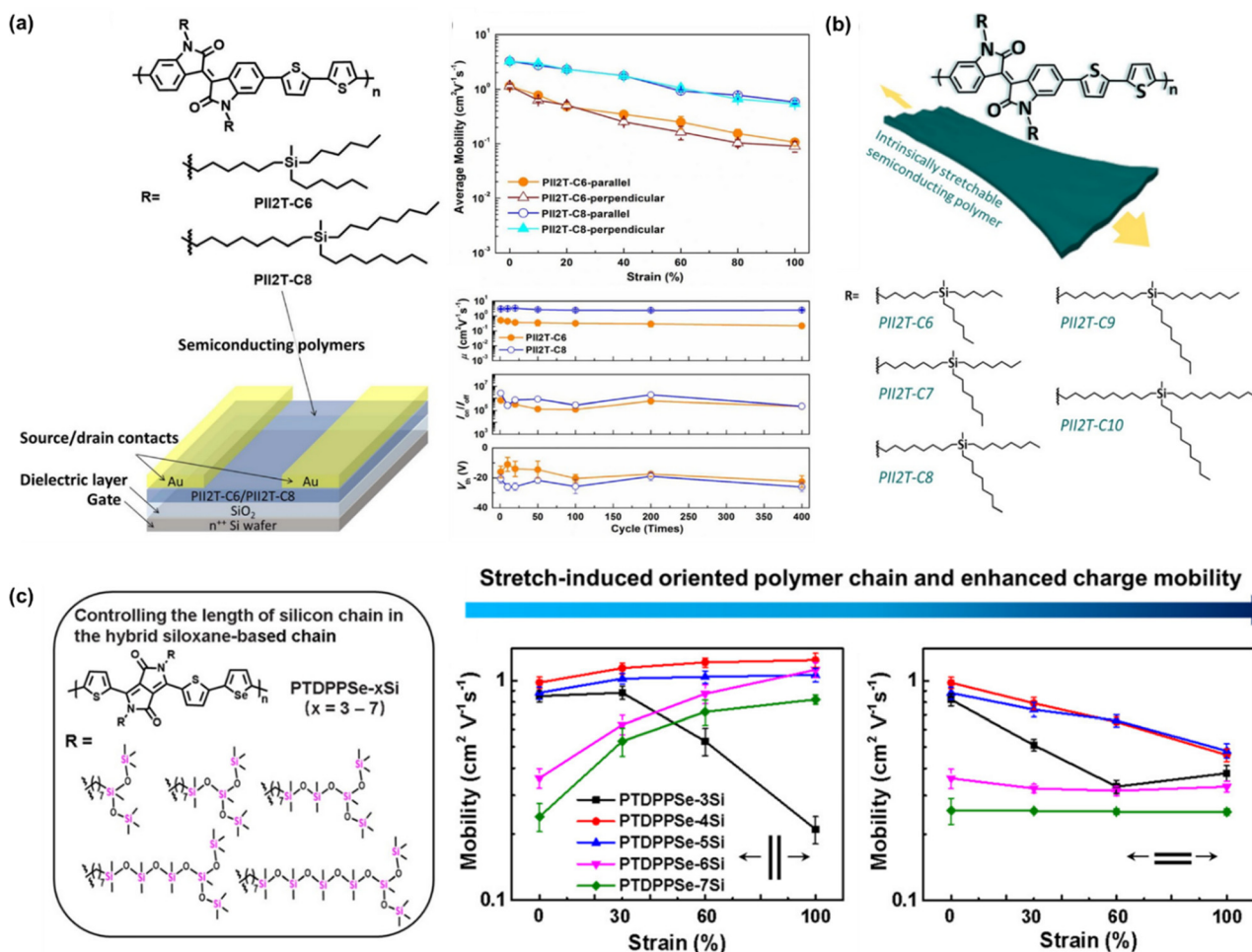
Fig. 8 Modulating the mechanical-electrical properties of conjugated polymers via side chain engineering based on \gamma -shaped approach. (a) Average field-effect mobility stretched in the parallel and perpendicular directions and the mechanical-mobility resistance of the PII2T-C6 and PII2T-C8 thin films under repeated 400 stretching/releasing cycles with a maximum strain of 60% controlled parallel to the strain direction. 113 Copyright: 2016, the American Chemical Society. (b) Chemical structures of PII2T-based polymers with manipulated length of carosilane side chains, charge mobility distribution in both parallel and perpendicular directions of PII2T with carbon position ranging from C6 to C10 and normalized mobility in the parallel direction of the studied polymer thin films under strain. 114 Copyright: 2019, the American Chemical Society. (c) PTDPpSe-based conjugated polymer bearing different lengths of silicon chain. 119 Copyright: 2022, the American Chemical Society.
