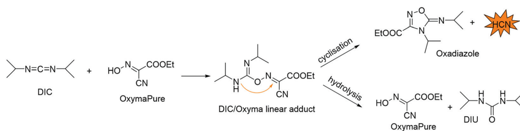
Fig. 13 Schematic representation of reactions involving Fig. 13 DIC and OxymaPure® to form a linear adduct and consequent possible formation of HCN. Note: DIU = diisopropyl urea.
