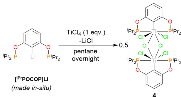
Scheme 5 Synthesis of 4.
