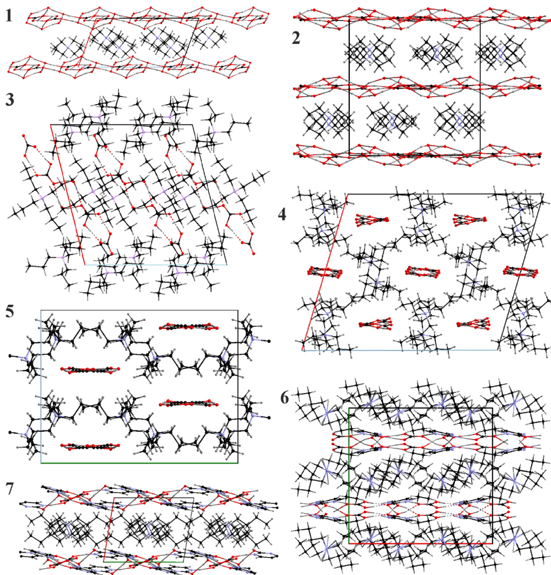
Fig. 3 Packing of the cations and the anionic fragments in the crystal structures of [\text{N}_{2222}][\text{HCO}_3] \cdot 3\text{H}_2\text{O} (1), [\text{N}_{2222}][\text{H}(\text{HCO}_3)_2] \cdot 5\text{H}_2\text{O} (2), [\text{N}_{3333}][\text{HCO}_3] \cdot 0.5\text{H}_2\text{O} (3), [\text{N}_{3333}][\text{H}(\text{HCO}_3)_2] (4), [\text{N}_{3333}]_2[\text{tpa}(\text{H}_2\text{CO}_3)_2] (5), [\text{N}_{4444}][\text{H}(\text{Cyt})(\text{HCO}_3)] \cdot \text{H}_2\text{O} (6) and [\text{N}_{4444}][\text{H}_2(\text{Cyt})_2(\text{HCO}_3)] \cdot \text{H}_2\text{O} (7).
