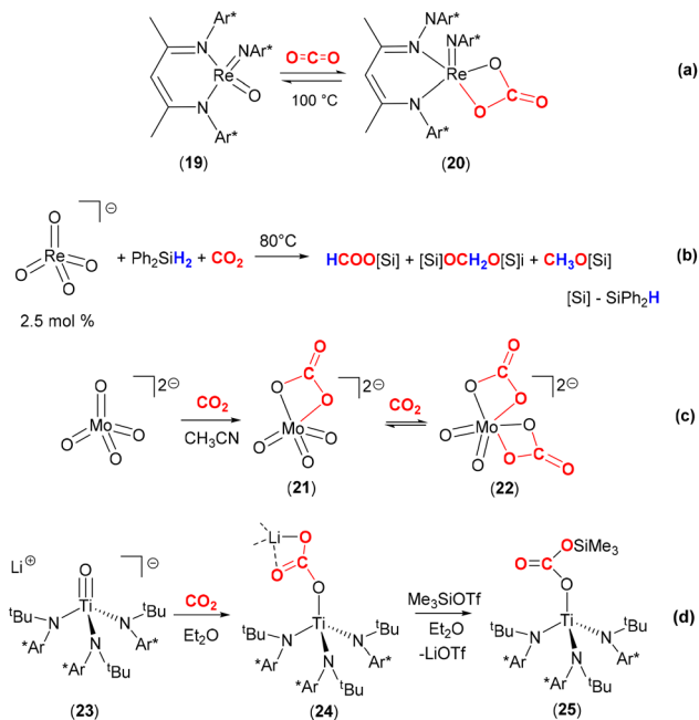
Scheme 4 Reaction of high valent early transition oxo complexes with \text{CO}_2 . \text{Ar}^* = 2,6 -diisopropylphenyl (Dipp).
