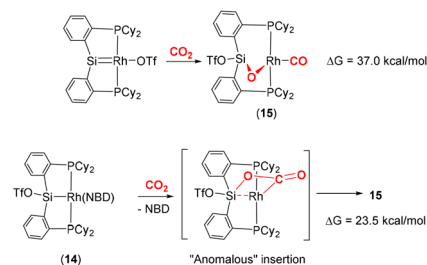
Scheme 3 DFT calculated pathways for \text{CO}_2 reductive cleavage of \text{CO}_2 into CO and siloxide by complex 14 . Top: silylene pathway, bottom: anomalous insertion pathway.
