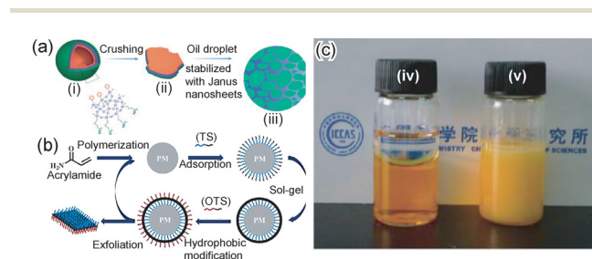
Fig. 2 (a) Scheme of the preparation of silica-based Janus nanosheets. Core-shell particles were formed by the self-assembly of three types of silica source and the sol-gel process at the water-oil interface in an emulsion. (i) After dissolution of the oil core, hollow silica spheres were formed. (ii) Silica-based Janus nanosheets were obtained by crushing the hollow silica spheres. (iii) The obtained silica-based Janus nanosheets can be used as a solid surfactant. 16 Adapted with permission from ref. 16. Copyright 2011 John Wiley and Sons. (b) Scheme of the preparation of silica-based Janus nanosheets via a reusable polyacrylamide microsphere template. 23 Adapted with permission from ref. 23. Copyright 2019 Elsevier. (c) (iv) An immiscible mixture of toluene (top) and water (bottom) and (v) a water-in-toluene emulsion stabilized with silica-based Janus nanosheets containing 69.6 wt% PDVB. 43 Adapted with permission from ref. 43. Copyright 2012 American Chemical Society.
