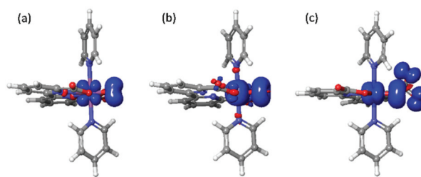
Fig. 4 Spin density distributions of [\text{Ru}^V(\text{bda})(\text{py})_2-\text{O}]^+ (left), [\text{Fe}^V(\text{bda})(\text{py})_2-\text{O}]^+ (middle) and 6-coordinate [\text{Fe}^V(\text{bda})(\text{py})_2-\text{O}]^+ (right) at an iso-value of 0.005 electrons per bohr 3 .
