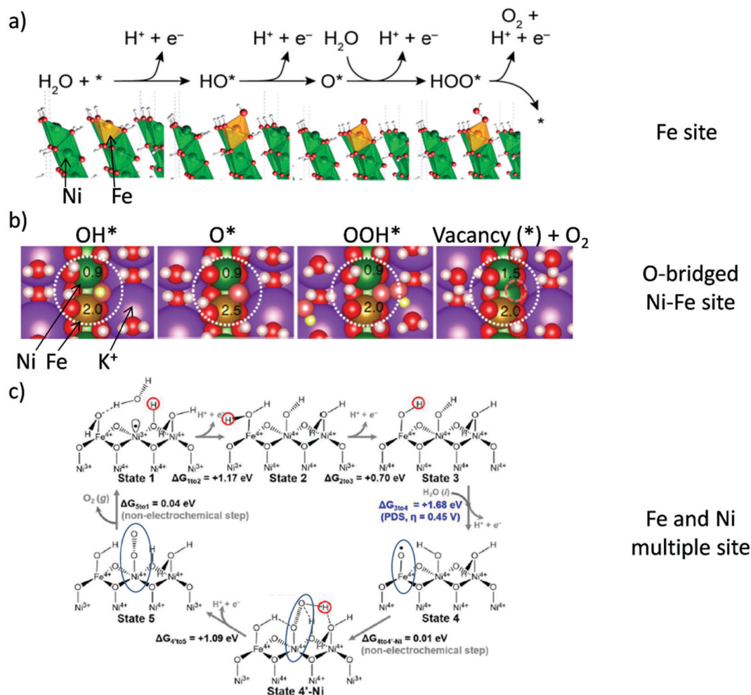
Fig. 52 NiFe (oxy)hydroxide active site and OER mechanism by DFT calculations. (a) Proposed OER pathway involving the \text{HO}^* , \text{O}^* and \text{HOO}^* intermediates and with a Fe atom site that was substituted in the (01 \bar{1} 2) surface of \gamma -NiOOH as the active site. Reproduced with permission from ref. 878. American Chemical Society. (b) A second proposed OER mechanism and intermediates on the H-saturated O-bridged Ni-Fe site as active site at the (01–10) surface of \gamma -NiFe LDH. The reaction centers are highlighted by large dotted white circles, the vacancy by a small pink dashed circle. The magnetic moments of Ni and Fe during OER are also given. Reproduced with permission from ref. 1775. Copyright Nature Publishing 2020. (c) A third example of proposed mechanism for OER on \text{Ni}_{1-x}\text{Fe}_x\text{OOH} catalyst. Blue ovals highlight the synergistic role of Ni and Fe sites in forming key reaction intermediates. Reproduced with permission from ref. 888. Copyright American Chemical Society 2018.
