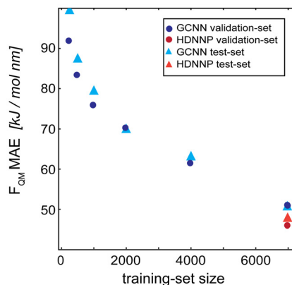
Fig. 9 Learning curves as a function of the training-set size of the \Delta -learning models for benzene in water (top) and uracil in water (bottom). The dark blue circles show the GCNN validation MAE, the dark red circles show the HDNNP validation MAE, the light blue triangles show the GCNN test MAE, and the light red triangles show the HDNNP test MAE. The numerical values are given in Table 3.
