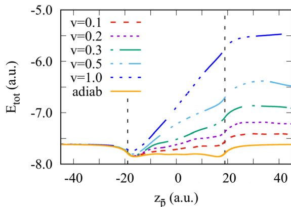
Fig. 1 Total energy of the Na 106 cluster as a function of the antiproton position. Different curves correspond to the results obtained for different antiproton velocities \nu as indicated in the insert, where \nu is given in atomic units. The orange curve denoted as “adiab” shows the adiabatic result. Vertical dashed lines indicate the border of the positive background of the jellium cluster.
