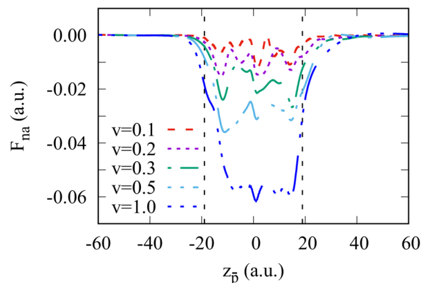
Fig. 3 Non-adiabatic force acting on the antiproton moving through the Na 106 cluster as a function of the antiproton position. Different curves correspond to the results obtained for different antiproton velocities \nu as indicated in the insert, where \nu is given in atomic units. Vertical dashed lines indicate the border of the positive background of the jellium cluster.
