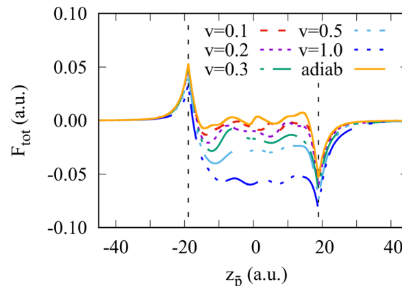
Fig. 2 Total force acting on the antiproton crossing the Na 106 clusters. Different curves correspond to the results obtained for different antiproton velocities \nu as indicated in the insert, where \nu is given in atomic units. The orange curve denoted as “adiab” shows the adiabatic result. Vertical dashed lines indicate the border of the positive background of the jellium cluster.
