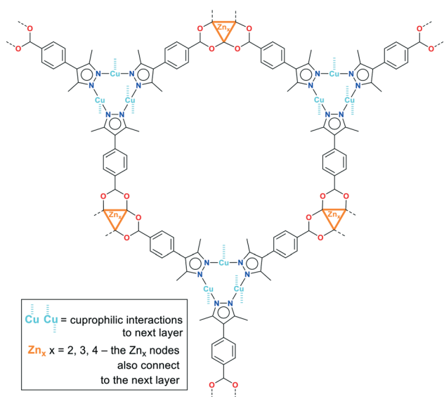
Scheme 2 Common features of the structures of 1–3 with Zn_x nodes of different nuclearities ( x = 2-4 ) and the trigonal \{Cu_3(\text{mpba})_3\}^{3-} nodes giving a hexagonal-ring layer. Both the Zn_x nodes and the cuprophilic interactions from \{Cu_3(\text{mpba})_3\}^{3-} connect to the next layer.
