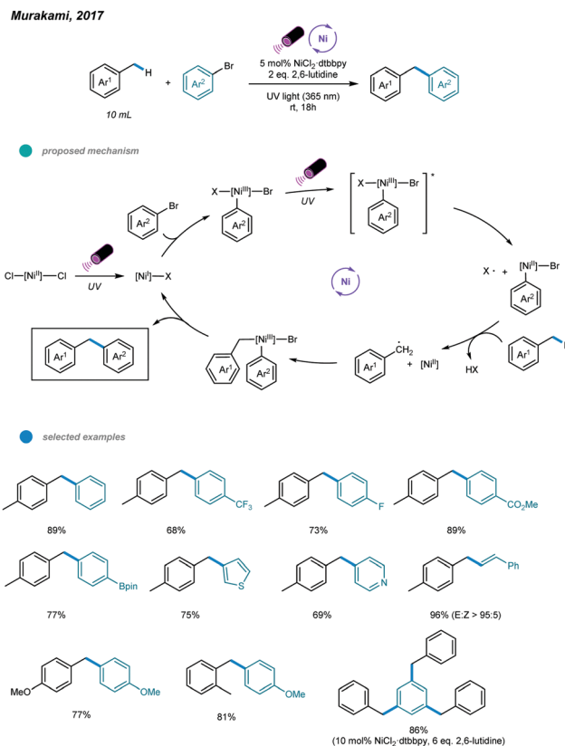
Scheme 3 UV light-induced nickel-catalyzed benzylic C–H arylations of methylbenzenes.
