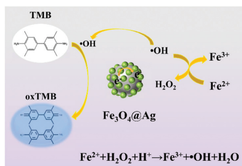
Scheme 1 An illustration of the catalytic oxidation of TMB by \text{Fe}_3\text{O}_4@\text{Ag} NPs.
