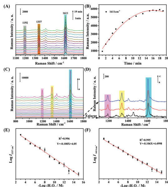
Fig. 4 (A) SERS monitoring of oxidized TMB molecules by \text{H}_2\text{O}_2 catalyzed by \text{Fe}_3\text{O}_4@\text{Ag} NPs. (B) The time-dependent variation of the SERS intensity of the band at 1611 \text{cm}^{-1} . (C) Concentration-dependent SERS spectra of TMB catalyzed by \text{Fe}_3\text{O}_4@\text{Ag} NPs in the presence of different concentrations of \text{H}_2\text{O}_2 (a: the blank sample; b–o: \text{H}_2\text{O}_2 concentration ranging from 10^{-15} to 10^{-3} M). (D) The enlarged spectra of a–c in the 1100–1800 \text{cm}^{-1} region in Fig. 4C. The plot of the logarithm of SERS intensities of the bands at 1337 \text{cm}^{-1} (E) and 1611 \text{cm}^{-1} (F) versus the logarithm of \text{H}_2\text{O}_2 concentrations.
