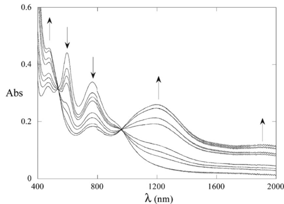
Fig. 18 Spectroelectrochemical reduction (0/–1 states) of complex 51 ( X = \text{tBuO} ) in THF and 0.2 M TBAPF 6 . Reproduced from ref. 150 with permission from the American Chemical Society.
