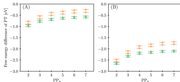
Fig. 6 Predicted free energy difference of proton transfer to the oligomer at the C 3 position as a function of oligomer length for PP n -H 2 O (A) and PP n -TEA (B), when TEA* + (upward triangle) and TEAR* (downward triangle) are the source of protons. B3LYP results in orange and CAM-B3LYP results in green.
