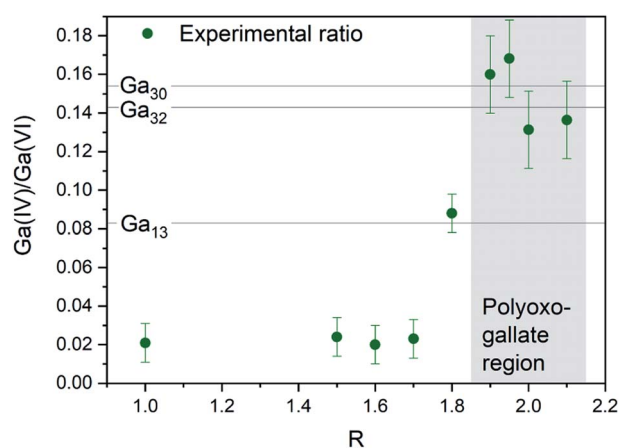
Fig. 7 Experimental ratios of the tetrahedrally to octahedrally coordinated \text{Ga}^{3+} determined by ^{71}\text{Ga} NMR. The horizontal lines indicate the ratios in the \text{Ga}_{13} , \text{Ga}_{30} and \text{Ga}_{32} structures at 0.083, 0.154 and 0.143 respectively. The grey area marks the R -region with the highest PDF signal from the polyoxogallate structure.
