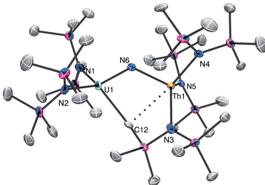
Fig. 2 Solid-state molecular structure of 3 shown with 50% probability ellipsoids. [K(18\text{-crown-6})]^+ cation, [K(18\text{-crown-6})(\text{Et}_2\text{O})_2]^+ cation, and hydrogen atoms removed for clarity. Selected bond lengths (Å) and angles ( ^\circ ): U1–N6 = 2.002(4), Th1–N6 = 2.160(5), U1–N1 = 2.366(5), U1–N2 = 2.349(5), Th1–N3 = 2.389(5), Th1–N4 = 2.395(5), Th1–N5 = 2.408(5), U1–C12 = 2.525(6), Th1–C12 = 2.962(5), U1–N6–Th1 = 122.2(2).
