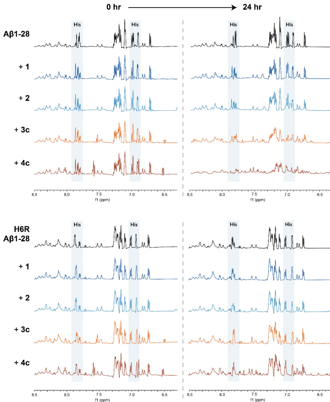
Fig. 5 ^1\text{H} NMR spectra of \text{A}\beta 1\text{-}28 (top) or H6R \text{A}\beta 1\text{-}28 (bottom) incubated by itself (black), with square planar 1 and 2 (blue) or octahedral 3c and 4c (orange) complexes (in a 1-to-1 \text{A}\beta -to-complex ratio). All spectra were recorded in \text{D}_2\text{O} : phosphate buffer (1 : 9, pH 7.4) at 37^\circ\text{C} and the spectra at 0 h and 24 h incubation time are shown. Peaks corresponding to the \text{A}\beta histidine residues are highlighted in blue.
