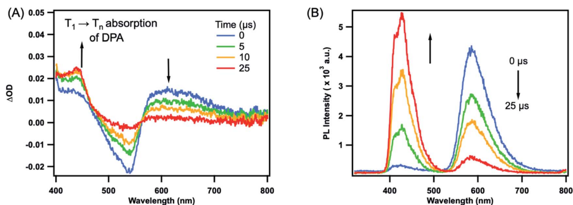
Fig. 3 Transient absorption difference spectra (A), and time-resolved photoluminescence spectra (B) of Zr( Mes PDP Ph ) 2 ( OD_{514 \text{ nm}} = 0.4 ) and 0.25 \text{ mM} DPA in deaerated THF at several delay times following 514 \text{ nm} pulsed laser excitation ( \sim 2 \text{ mJ} per pulse) with delay times indicated.
