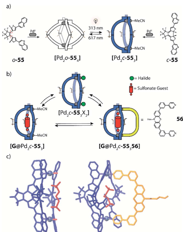
Fig. 27 (a) Photoswitching a quinolinyl-substituted ligand with dithienylethene (DTE) backbone allows cycling between a [Pd 2 L 4 ] cage and [Pd 2 L 3 Solv 2 ] bowl-shaped structure; (b) guest binding can be modulated by changing the host's charge from 4+ to 2+ by adding halide anions as trigger or by changing the cavity size via a fourth ligand (yellow); (c) X-ray crystal structures of host-guest complexes of the bowl and unprecedented [Pd 2 L 3 L] heteroleptic cage.
