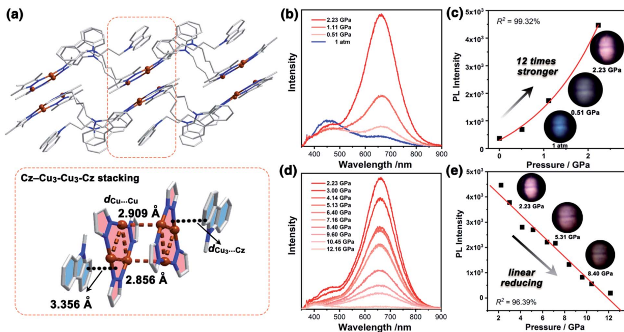
Fig. 1 (a) The crystal packing of 1a at 100 K, showing discrete C z -Cu 3 -Cu 3 -C z stacking (Cu: brown, C: grey, and N: blue, H atoms are omitted for clarity). Emission spectra of 1a at a range of external pressures from (b) 1 atm–2.23 GPa and (d) 2.23–12.16 GPa at an excitation wavelength of 355 nm. The curve fitting [function: y = A_1 \times \exp(-x/t_1) + y_0 , R^2 = 99.32\% ] and linear fitting [function: y = A_0 + kx , R^2 = 96.39\% ] of pressure and PL intensity for 1a in pressure ranges of (c) 1 atm–2.23 GPa and (e) 2.23–12.16 GPa (insets of (c) and (e): PL photographs at representative pressure points).
