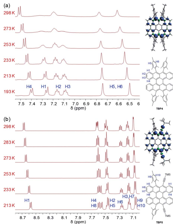
Fig. 4 VT ^1\text{H} -NMR spectra of (a) TBP4 and (b) TBP5 in DCM- d_2 in the aromatic region.
