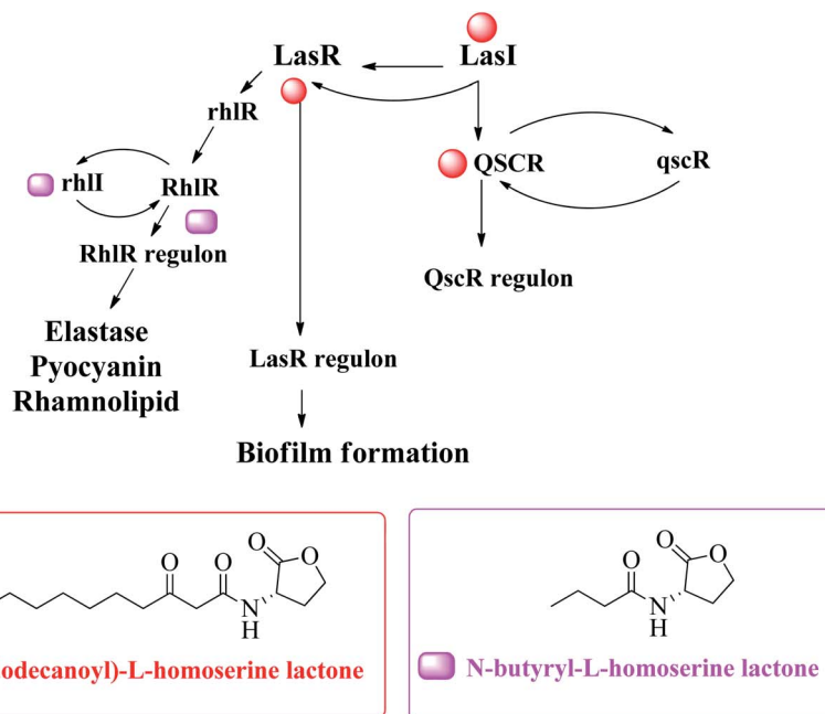
Fig. 10 A hypothetical model explaining transcriptional regulation of QSI in P. aeruginosa . 82
