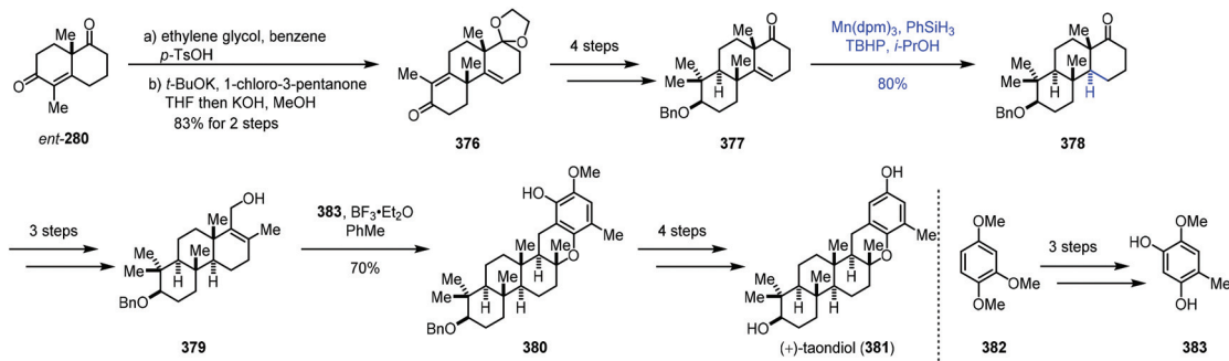
Scheme 47 Dethe's synthesis of (+)-taondioid (381).
