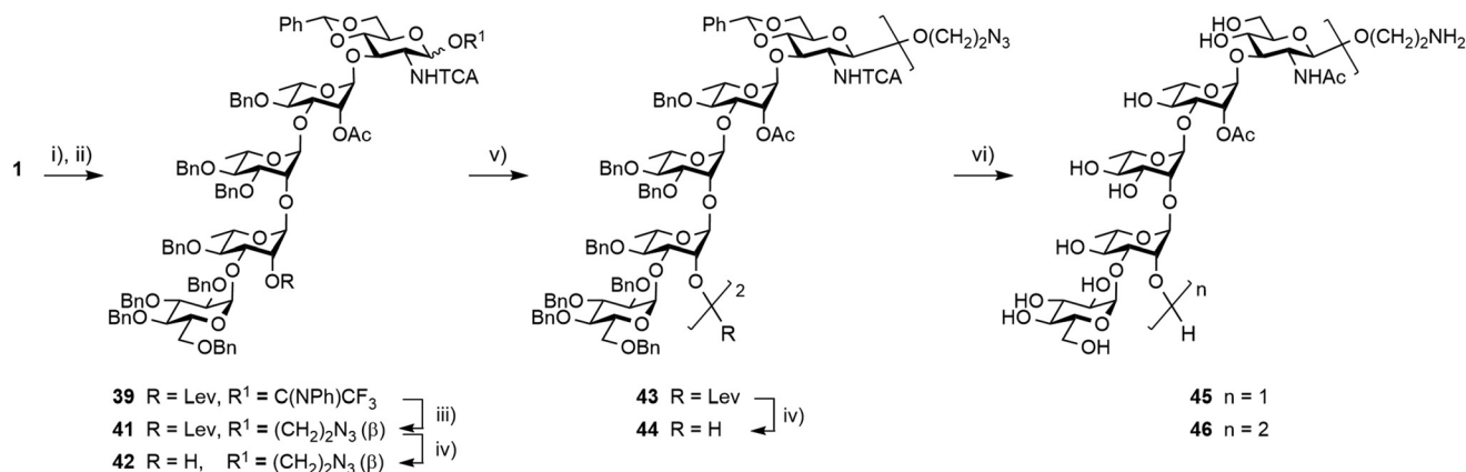
Scheme 10 Synthesis of decasaccharide 46 from the pentasaccharide building block 1 . (i) [Ir(COD)](PCH 3 (C 6 H 5 ) 2 ) 2 + PF 6 − , THF, then I 2 , THF/H 2 O; (ii) PTFACl, K 2 CO 3 , acetone, 0 °C, 88% (over 2 steps); (iii) 2-azidoethanol, TMSOTf, toluene, −40 °C, 78%; (iv) NH 2 NH 2 ·H 2 O, pyridine/AcOH (3 : 2), 91% for 42 and 92% for 44 ; (v) 39 (1.3 equiv.), 4 Å MS, toluene, −40 °C, 88%; (vi) Pd(OH) 2 , H 2 , tBuOH/DCM/H 2 O, 70% for 45 from 42 , 52% for 46 from 44 .
