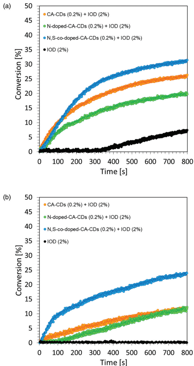
Fig. 10 Free-radical photopolymerization profiles (acrylate function conversion vs. irradiation time) for TMPTA with the bimolecular photoinitiating system based on IOD (2.0 wt%) and CD (0.2 wt%) (a) under irradiation at 365 nm; (b) under irradiation at 405 nm. Irradiance was measured at a distance of 210 mm for all sources.
