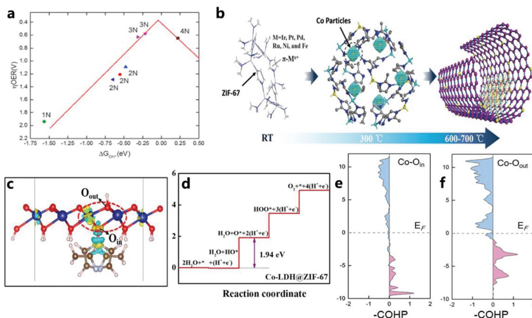
Fig. 23 (a) ZIF-67- x\text{N} ( x = 1\text{--}4 ) volcano diagram related to the OER catalytic activity and OH adsorption energy on the Co site. 138 Copyright © 2017 Elsevier Ltd. All rights reserved. (b) Illustration of locations of metal cations and \pi electrons. (At room temperature, metal cations are initially related to \pi electrons. At 300 °C, the metal atoms embedded in cobalt form single atoms. At 600–700 °C, cobalt forms on the base carbon atom.) 137 Copyright © 2019 Wiley-VCH Verlag GmbH & Co. KGaA, Weinheim. (c) The charge density difference of the underlying layer for Co-LDH@ZIF-67, and (d) the Gibbs free energy step diagram of the OER on Co-LDH@ZIF-67. pCOHP for (e) Co-O in and (f) Co-O out in Co-LDH@ZIF-67. 187 Copyright © 2020 The Authors. Published by Wiley-VCH GmbH.
