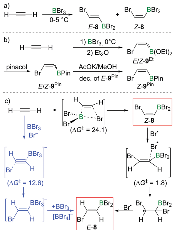
Scheme 8 (a) Reaction of acetylene with BBr 3 . (b) Brønsted-acid-free workup conditions allow for the selective isolation of Z-9 Pin . (c) Possible reaction pathways and energies (kcal mol -1 ) of acetylene bromoboration.
