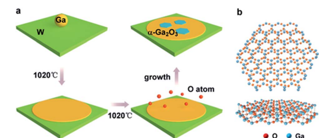
Fig. 1 (a) Schematic of the \alpha -Ga 2 O 3 structure growth process. A drop of liquid Ga is placed on a W substrate. Then the Ga forms a flat surface owing to the good wetting behavior between Ga and the substrate as the temperature is increased. The O atoms diffuse to the surface of the liquid Ga to react and form hexagonal-shaped \alpha -Ga 2 O 3 . (b) Crystal configuration of an \alpha -Ga 2 O 3 flake.
