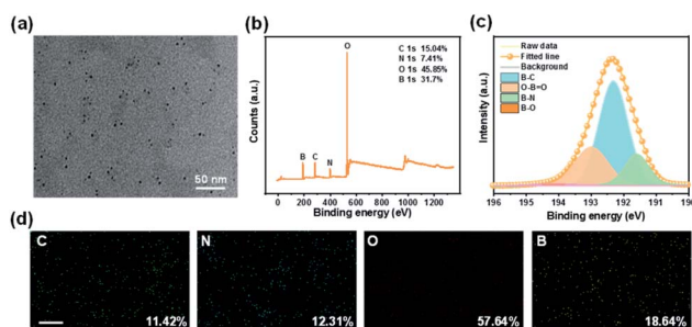
Fig. 2 (a) TEM image of CD/BNO. (b) XPS spectra of CD/BNO. (c) XPS high-resolution B 1s spectra of CD/BNO. (d) Energy-dispersive X-ray spectroscopy (EDS) mapping images of CD/BNO, scale bar is 5 \mu m.
