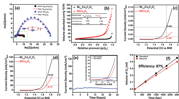
Fig. 4 (a) Nyquist plots of different electrocatalysts, (b) \text{N}_2 adsorption-desorption isotherm of \text{Ni}_{2.5}\text{Co}_5\text{C}_2\text{O}_4 and \text{NiCo}_2\text{O}_4 samples, catalytic performance in terms of (c) BET surface area normalised LSV plot and (d) geometrical area normalised LSV plot for \text{Ni}_{2.5}\text{Co}_5\text{C}_2\text{O}_4 and \text{NiCo}_2\text{O}_4 samples, (e) stability study of the best catalyst \text{Ni}_{2.5}\text{Co}_5\text{C}_2\text{O}_4 [the inset showing the overpotential value to reach the benchmark of 10 \text{ mA cm}_{\text{geo}}^{-2} ], and (f) analysis of faradaic efficiency for the \text{Ni}_{2.5}\text{Co}_5\text{C}_2\text{O}_4 .
