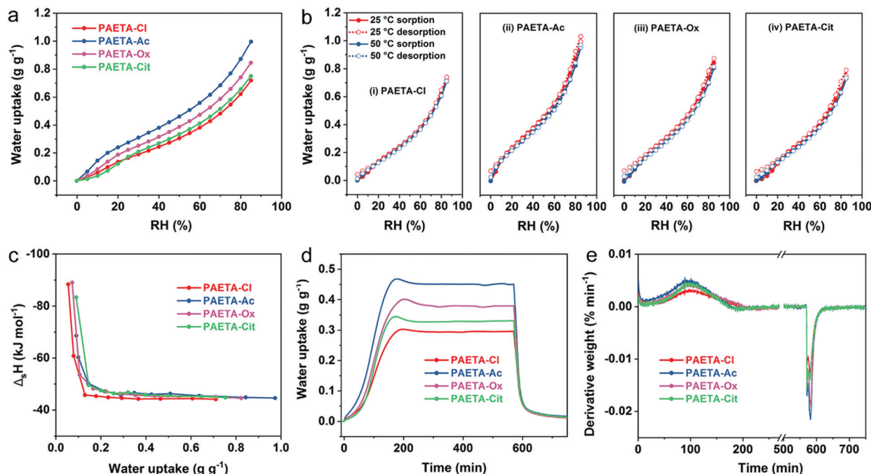
Fig. 3 (a) Water vapor sorption isotherms at 25 °C, (b) water vapor sorption and desorption isotherms at 25 °C and 50 °C, (c) \Delta H as a function of water uptake, (d) static water sorption-desorption curves, and (e) 1st derivative curves of static water sorption-desorption for PAETA-X hydrogels.
