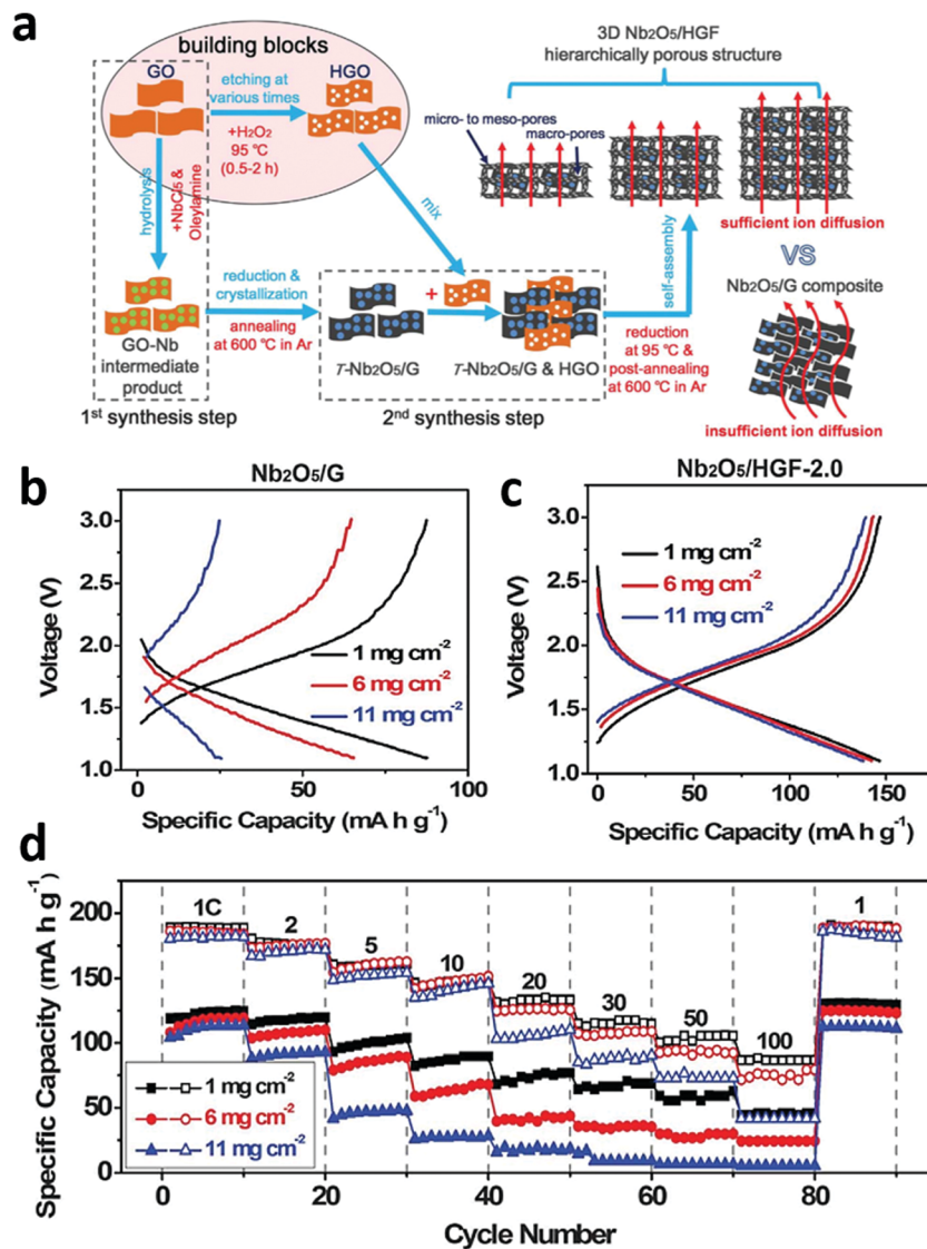
Fig. 12 (a) Illustration of the two-step synthetic procedure to prepare a 3D T-Nb _2\text{O}_5/\text{HGF} composite. Galvanostatic charge–discharge curves of (b) the Nb _2\text{O}_5/\text{G} electrode, and (c) the Nb _2\text{O}_5/\text{HGF}-2.0 electrode at 10.0^\circ\text{C} for mass loadings of 1, 6, and 11 \text{mg cm}^{-2} , respectively. (d) Comparison of the rate performance between 1.0C and 100.0C for Nb _2\text{O}_5/\text{HGF}-2.0 and Nb _2\text{O}_5/\text{G} electrodes under different mass loadings. Reprinted with permission from ref. 129. Copyright 2017, Science.
