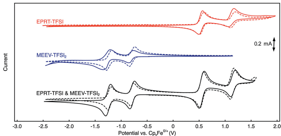
Fig. 4 Cyclic voltammograms of EPRT-TFSI (red, top traces), MEEV-(TFSI) 2 (blue, middle traces), and an equimolar combination of both EPRT-TFSI and MEEV-(TFSI) 2 (black, lower traces) at 10 mM in ACN with no supporting salts (solid-line) and in ACN with 0.5 M TEATFSI (dashed-line). CV experiments were performed at a scan rate of 100 mV s -1 , and 100% iR correction was applied. All voltammograms are referenced to ferrocene/ferrocenium at 0 V.
