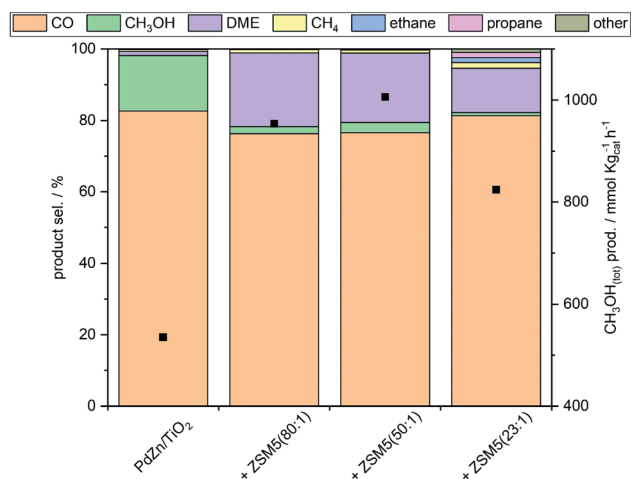
Fig. 3 CO, oxygenate and hydrocarbon selectivity and total \text{CH}_3\text{OH} productivity for \text{CO}_2 hydrogenation (20 bar, 270 °C, \text{CO}_2/\text{H}_2/\text{N}_2 = 1 : 3 : 1 ) over \text{PdZn/TiO}_2 and \text{PdZn/TiO}_2 -ZSM-5 hybrid catalysts.
