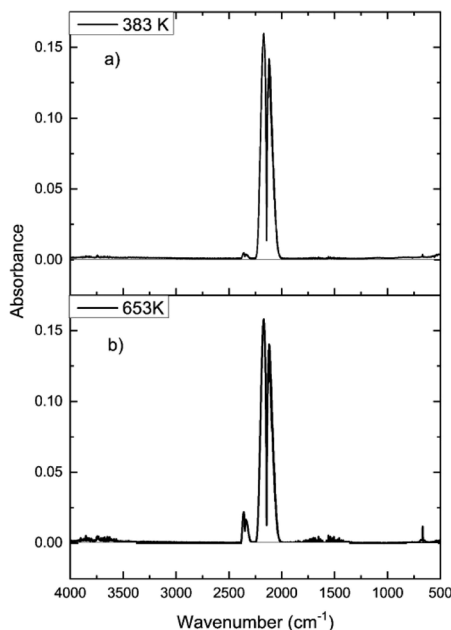
Fig. 11 FTIR spectra for continuous CO dosing over the dried support material (attapulgitite) at (a) 383 and (b) 653 K. Flow conditions: CO 5\text{ cm}^3\text{ min}^{-1} , N 2 (carrier gas) 54\text{ cm}^3\text{ min}^{-1} , and N 2 (diluent post-reactor) 100\text{ cm}^3\text{ min}^{-1} .
