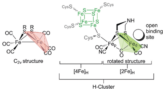
Fig. 8 H-cluster of [FeFe]-hydrogenases with indicated rotated motif of the distal iron atom (green) vs. the Fe_2S_2(CO)_6 core in C_{2v} symmetry (red).
