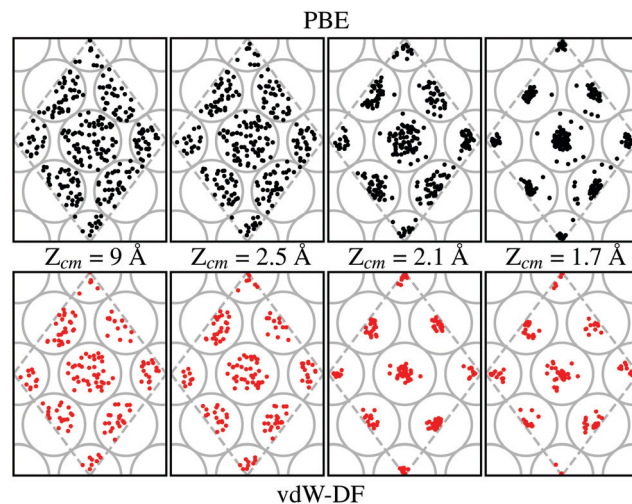
Fig. 7 Evolution of the molecules that eventually dissociate. Different vertical distances Z_{\text{cm}} are considered. Black and red dots represent the center of mass of molecules over the 2 \times 2 cell employed (gray dashed lines). Grey circles correspond to the W atoms of the surface. Upper panel corresponds to trajectories simulated using the PBE xc-functional. For the lower panels, vdW-DF xc-functional has been used. The initial collision energy is 200 meV for all trajectories.
