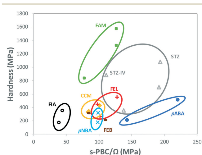
Fig. 4 Hardness measured with nanoindentation on various polymorphic systems as a function of the s-PBC normalised by the mean molecular volume \Omega . Circles contain data for individual polymorphic systems. The general trends per individual system show an increase in hardness with s-PBC, but such trend is less obvious when considering all systems together. We note that febusostat (FEB, brown symbols) is the only system for which the trend shows that lower hardness is obtained at higher value of s-PBC/ \Omega .
