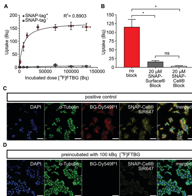
Fig. 2 In vitro binding study of [ ^{18}\text{F} ] FTBG to SNAP-tag + Gli36 cells. (A) 1 \times 10^5 SNAP-tag + or SNAP-tag - cells were incubated with a dilution series of [ ^{18}\text{F} ]FTBG for 30 min. Cells were washed, harvested and radioactivity bound to cells was measured with a gamma-counter. SNAP-tag + cells accumulate much higher amounts of radioactivity and approach a plateau-phase at higher concentrations of the ligand ( n = 4 , R^2 = 0.89 , B_{\text{max}} = 170.6 \pm 7.8 Bq, K_d = 7784 \pm 1605 Bq, non-linear regression analysis with one-side fit with total and non-specific binding) as compared to SNAP-tag - cells. (B) 1 \times 10^5 SNAP-tag + cells were incubated with cell-permeable SNAP-Cell ® or non-permeable SNAP-Surface ® block substrates or were left untreated before 100 kBq [ ^{18}\text{F} ]FTBG was added. Blocking resulted in significantly lower accumulation of radioactivity in the cells when compared to control cells ( n = 4 , RM One-way ANOVA with Tukey's test for multiple comparisons, * p < 0.05 ). (C) Labeling of SNAP-tag + Gli36 cells with fluorescent O^6 -benzylguanines. Labeling with cell-impermeable BG-Dy549P1 shows bright staining at the plasma membrane, incubation with cell-permeable SNAP-Cell ® 647-SIR stains intracellular and extracellular epitopes. (D) Fluorescent signals are strongly reduced when cells were first incubated with 100 kBq [ ^{18}\text{F} ]FTBG. Scale bars 100 μm. All data is shown as mean ± SEM.
