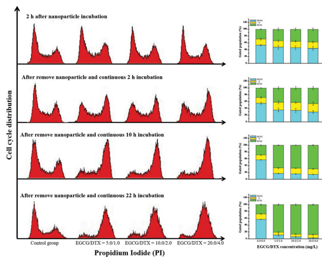
Fig. 6 The proportions of cells in the G0/G1, S, and G2/M phases was analyzed using flow cytometry after treatment with EGCG/DTX-loaded TPGS- g -HA/FD/PEG- g -GE nanoparticles for different incubation times.
