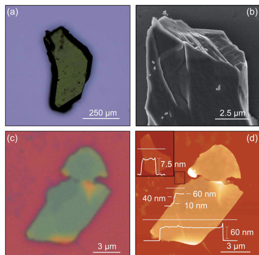
Fig. 5 The laminar structure of 2-bpy \sigma revealed by imaging pre- and post-mechanical exfoliation of a single crystal. (a) Optical microscopy image of a bulk single crystal. (b) Scanning electron microscopy image focused on laminar edge of the bulk crystal. (c) Optical microscopy of a mechanically exfoliated flake. (d) Atomic force microscopy characterization of the exfoliated flake, including height profiles and a zoom-in inset of a thin flake.
