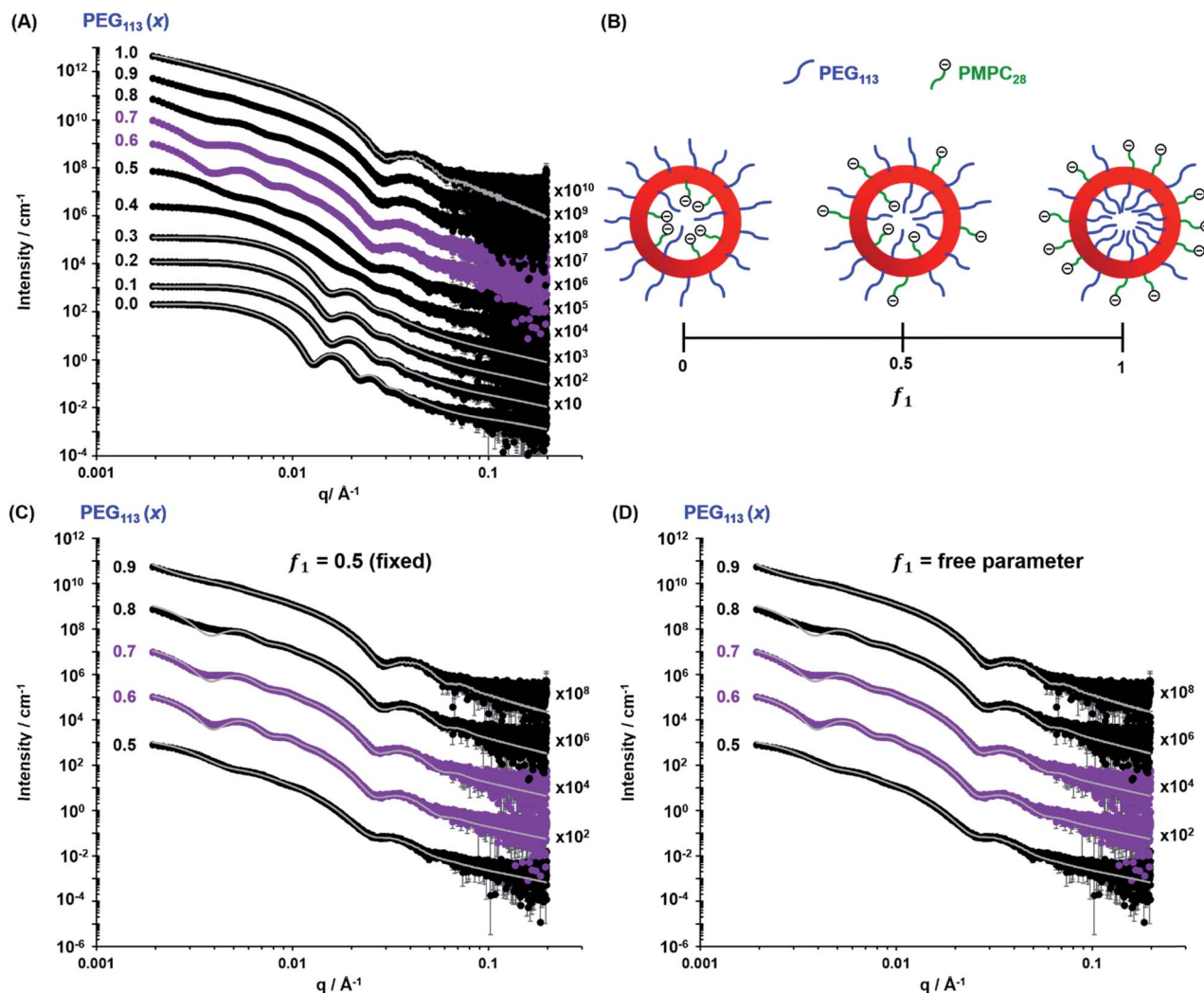
Fig. 4 (A) Experimental SAXS patterns (symbols) and corresponding data fits (grey lines) obtained for 1.0% w/w aqueous dispersions of [x \text{ PEG}_{113} + (1-x) \text{ PMPC}_{28}] - \text{PPHMA}_{400} nano-objects originally prepared at 10% w/w solids, where the mole fraction ( x ) ranges from 0.0 (PMPC 28 -PPHMA 400 ) to 1.0 (PEG 113 -PPHMA 400 ). Scattering curves obtained for nano-objects prepared using a PEG mole fraction of 0.1–0.3 could be satisfactorily fitted using the blob-modified spherical micelle model, while the scattering patterns obtained for PMPC 28 -PPHMA 400 spheres were fitted using a well-known spherical micelle model. 100 A well-established vesicle model 101 was employed to fit the scattering pattern recorded for PEG 113 -PPHMA 400 vesicles obtained when x = 1.0 . (B) Schematic representation of the segregation fitting parameter f_1 , which indicates the mole fraction of PMPC 28 chains occupying the outer leaflet of the vesicles. (C) Experimental SAXS patterns [same symbols as shown in (A)] recorded for the sub-set of [x \text{ PEG}_{113} + (1-x) \text{ PMPC}_{28}] - \text{PPHMA}_{400} vesicles obtained for x = 0.50 - 0.90 . These patterns were fitted using a refined vesicle model that takes account of the binary mixture of diblock copolymer chains [eqn (16)] using a fixed segregation parameter f_1 of 0.50 (which corresponds to a purely statistical mixture of PEG and PMPC stabilizer chains occupying the outer corona). The grey lines indicate the data fits obtained using this more sophisticated scattering model. In contrast, (D) shows the data fits obtained when f_1 is allowed to vary as a free parameter.
