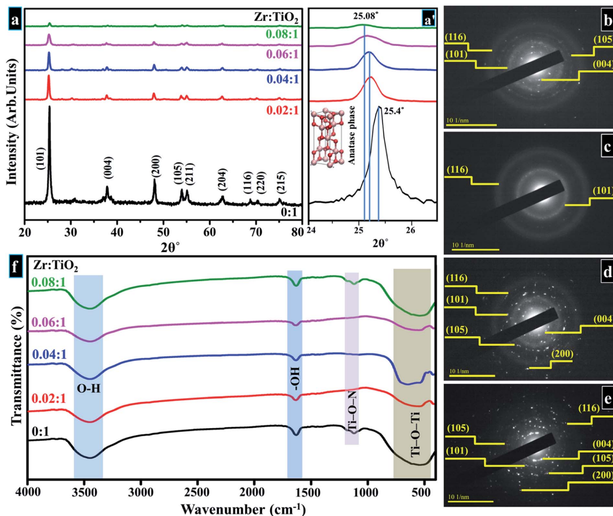
Fig. 5 (a) XRD pattern (a') zoomed area of (101) plane (b–e) SAED profiles of as-prepared and Zr-doped \text{TiO}_2 , respectively (f) FTIR spectra.
