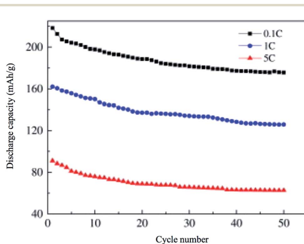
Fig. 17 Cyclic performance of nano \text{C}/\text{Li}_2\text{MnSiO}_4 synthesized by ionothermal method, the material is tested in the potential range of 2.5–4.5 V. 153
