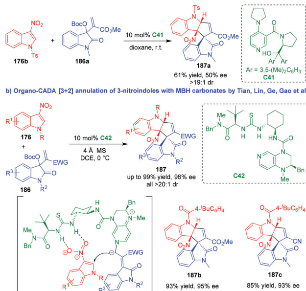
Scheme 44 Organo-CADA [3 + 2] annulation of 3-nitroindoles with MBH carbonates. 83,84
