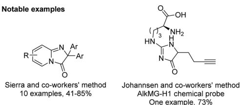
Scheme 11 General condensation of diketone and amidine to produce di- and tri-substituted imidazol-4-ones.
