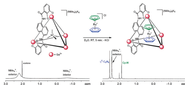
Fig. 4 NMe_4^+ guest exchange with 2, K_6(NMe_4)_5[II_{Ga}^e-NMe_4] before (left), and after (right) the addition of [CpRu(\eta^6-C_6H_6)]^+ . Reproduced with permission from ref. 47. Copyright 2004, American Chemical Society.
