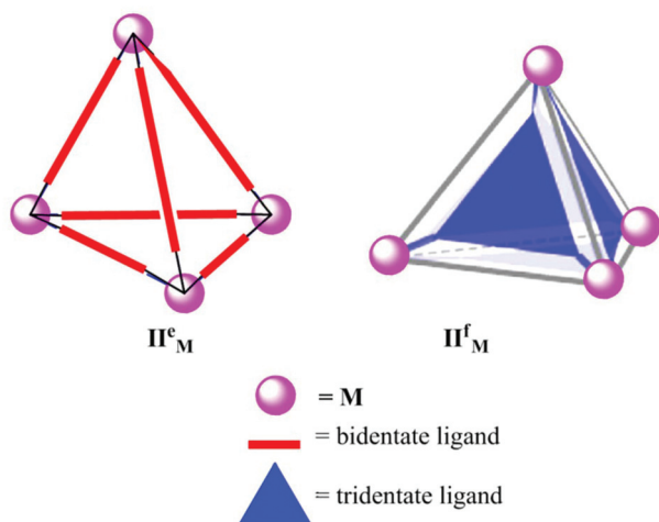
Fig. 3 Representation of two types of tetrahedral cages ( II_M^e and II_M^f ) synthesized using bis-bidentate ( M_4L_6 ) and tridentate ( M_4L_4 ) ligands, respectively.
