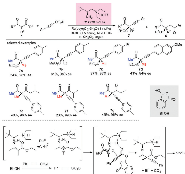
Scheme 48 Asymmetric alkynylation via primary amine-photocatalysis.
