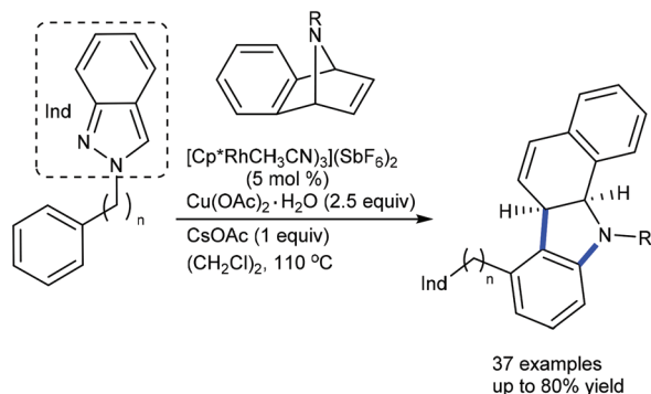
Scheme 132 Coupling of aryl-2 H -indazoles with 7-azabenzonorbornadiene.
